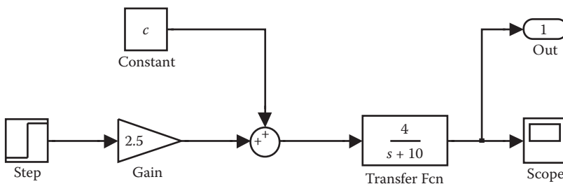
FIGURE 10.18 Simulink block diagram of open-loop control with disturbance input.
