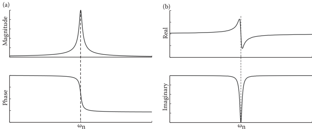
FIGURE 9.27 Frequency response of a single-degree-of-freedom system represented in terms of (a) magnitude and phase, and (b) real and imaginary.
